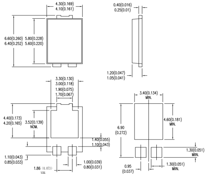
TO-277B
